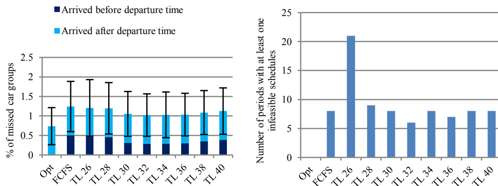
Figure 5: Left: The average percentage of missed cars for the stochastic simulation for all planning methods. Error bars show the standard deviation. Right: The number of periods (out of 21) for the stochastic simulation where at least one of the simulation runs resulted in an infeasible allocation being generated.
